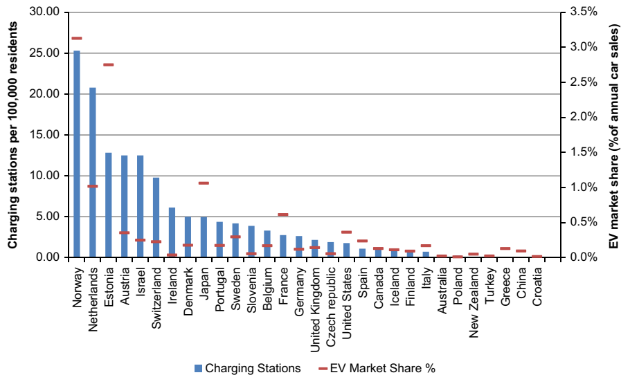
Fig. 3. National charging infrastructure by country and corresponding EV market share for 2012.
